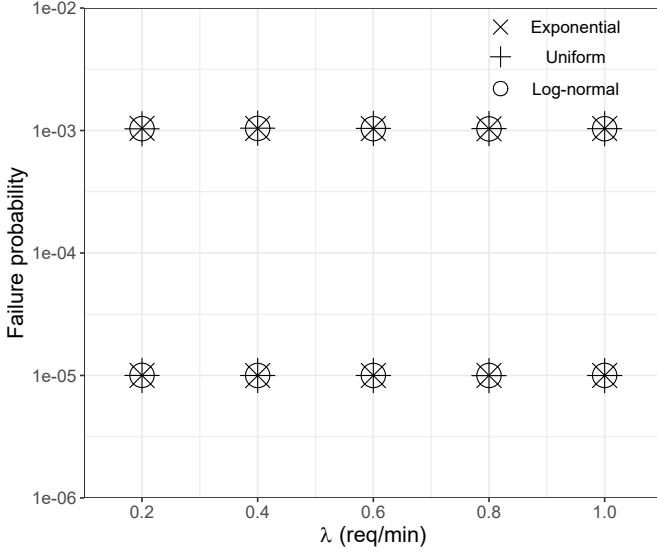
Fig. 3: Failure probability vs. \lambda for two target values, 10^{-3} (top) and 10^{-5} (bottom), and different service times.
