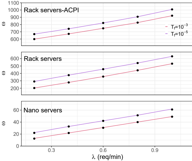
Fig. 4: Power consumption vs. \lambda . Lines represent the consumption of A3S. Points give the consumption resulting from performing an exhaustive search and selecting the best configuration.
