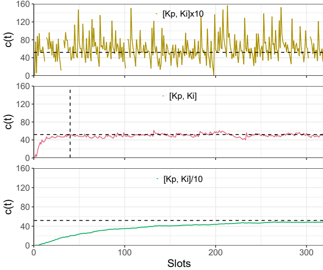
Fig. 5: Behavior of the control signal for different configurations of the controller parameters.
