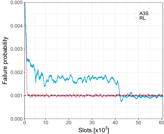
Fig. 7: Comparison of A3S and RL: failure probability over time. The figure shows that A3S converges much more quickly than Reinforcement-Learning (RL).
