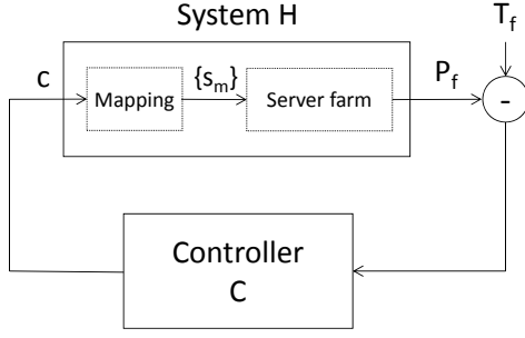
Fig. 1: Closed-loop system.
