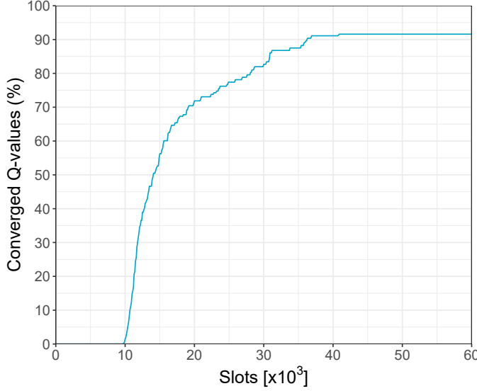
Fig. 6: Convergence of the Q-values for the Reinforcement-Learning (RL) technique: percentage of Q-values that have converged as a function of time.
